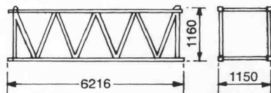
③ - 2 20 ft boom insert 734 kg
