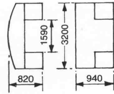
Counterweight (C) - 8,800 Kg
