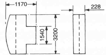
Counterweight (A) - 4,000 Kg
