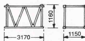
③ - 1 10 ft boom insert 411 kg
