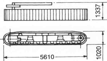
② Side frames - 8,900 Kg x 2
