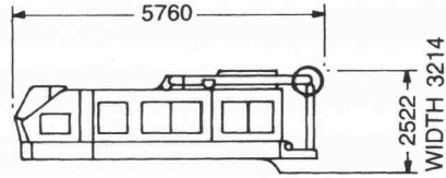
① - 2 Superstructure (with gantry) - 21,600 Kg
