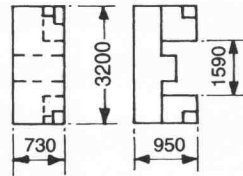
Counterweight (B) - 8,800 Kg
