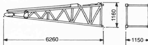
① Lower boom - 20 ft 2,300 Kg
