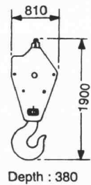
④ 75 - tonne hook block 998 kg
