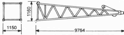
② Upper boom - 30 ft 2,280 kg
