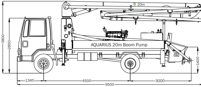
Reach Diagram 20m Boom
