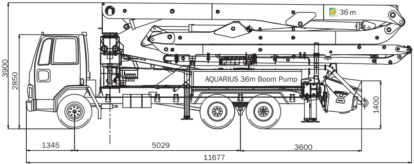
Reach Diagram 36m Boom
